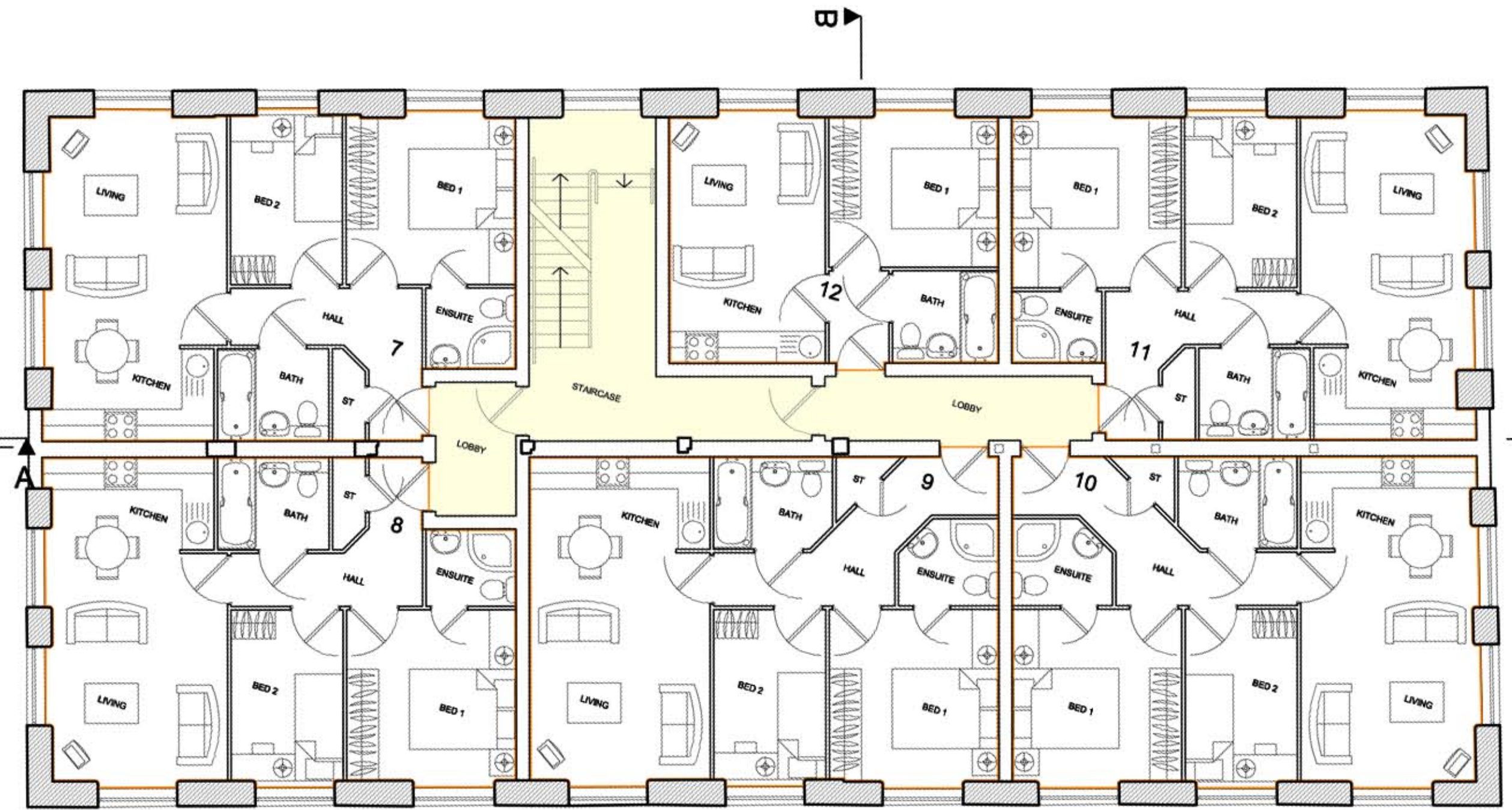
FIRST FLOOR
