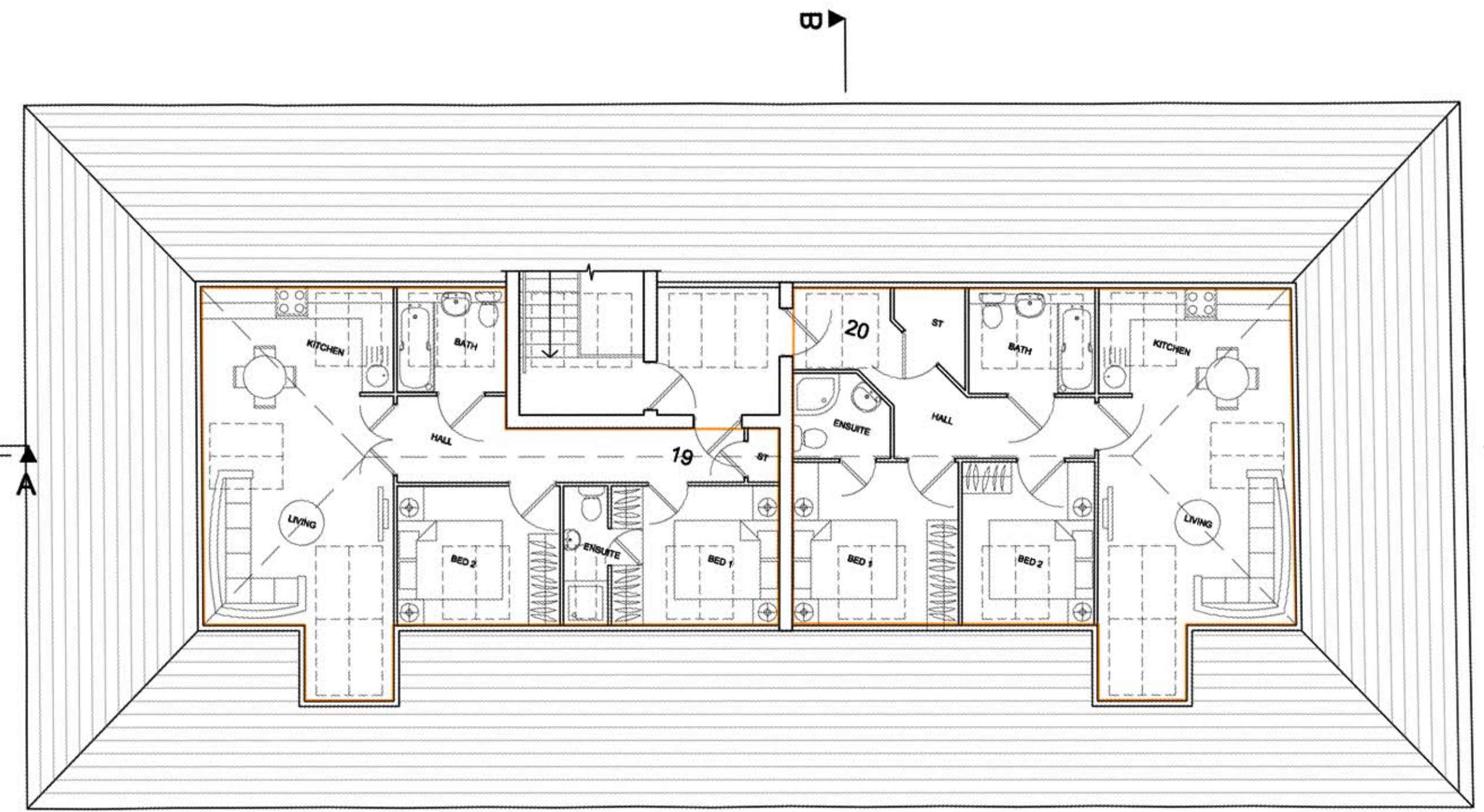
THIRD FLOOR
